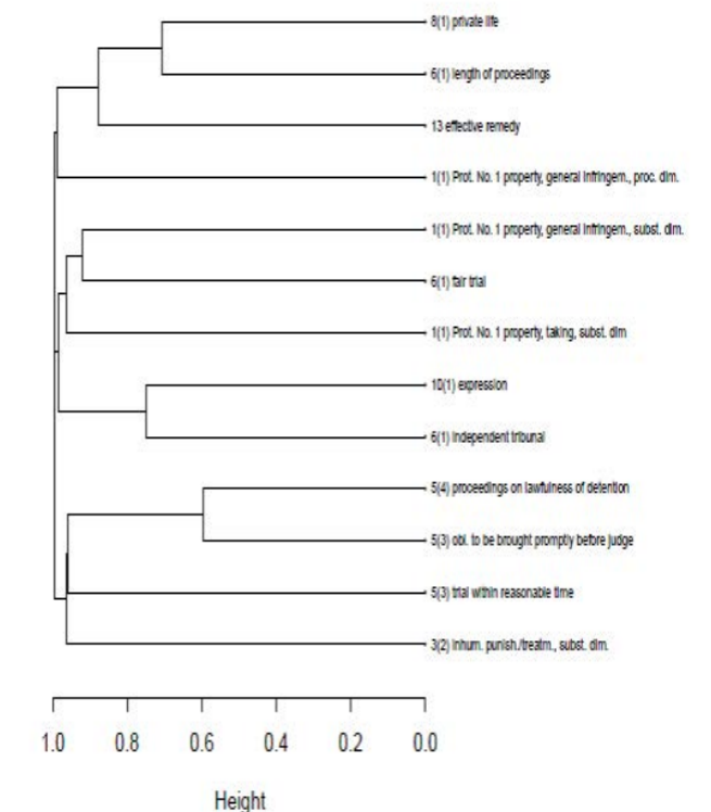
Hierarchical Cluster Analysis of violated ECHR Articles (N=1685)
